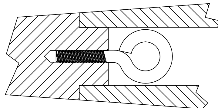
1/4-20 Stainless Eyebolt McMaster Carr PN: 9489T56
